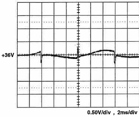
+36V step from 1.12A to 5.6A
