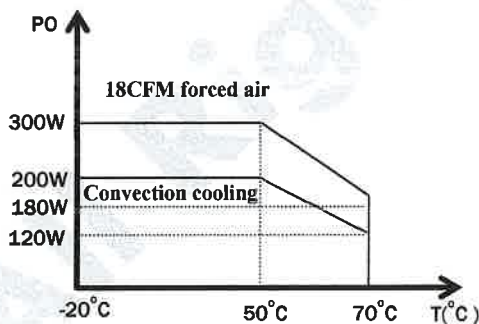
Output derating curve
