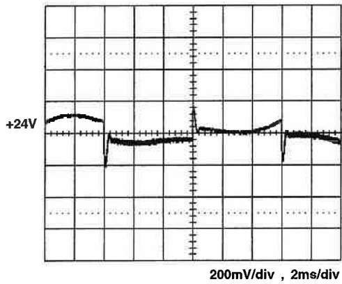
+24V step from 1.68A to 8.4A
