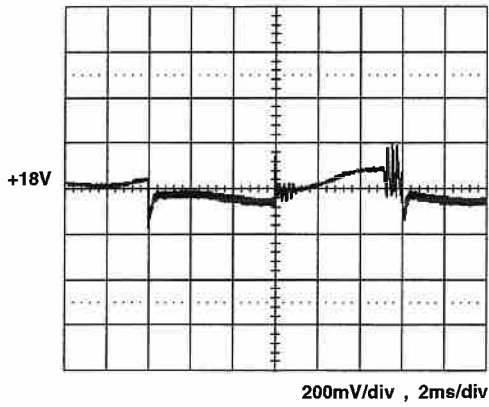
+18V step from 2.22A to 11.1A
