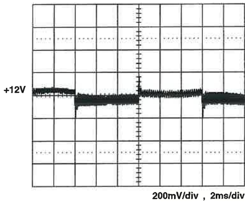
+12V step from 4.95A to 16.5A
