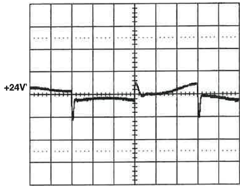
+24V step from 1.998A to 6.66A
