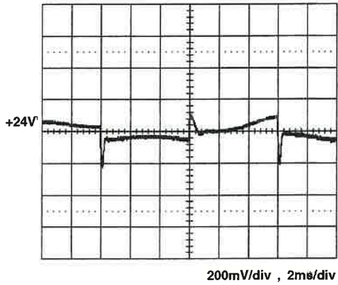
+24V step from 1.998A to 6.66A
