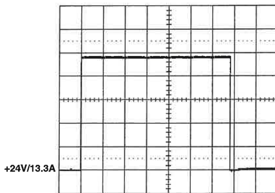
5.0V/div , 2s/div
