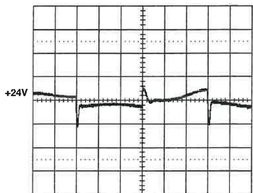
200mV/div , 2ms/div
