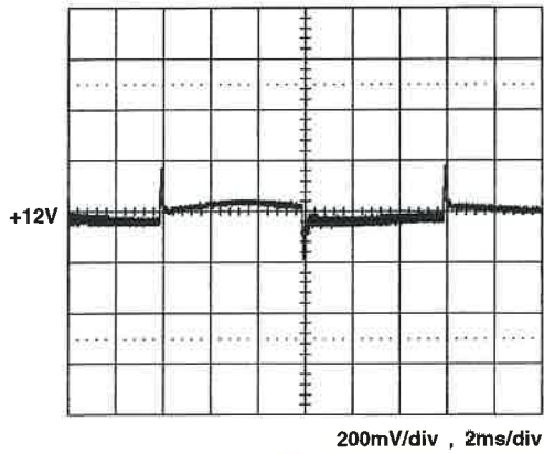
+12V step from 3.99A to 13.3A
