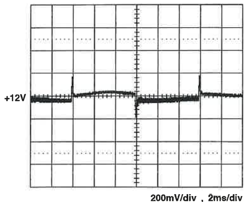
+12V step from 3.99A to 13.3A
