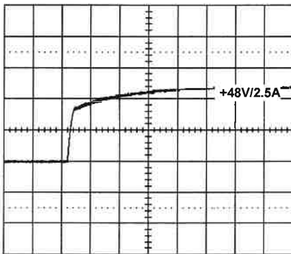
20.0v/div , 20ms/div
