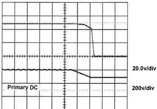
20ms/div
