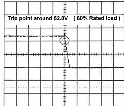
20.0V/div , 20ms/div
