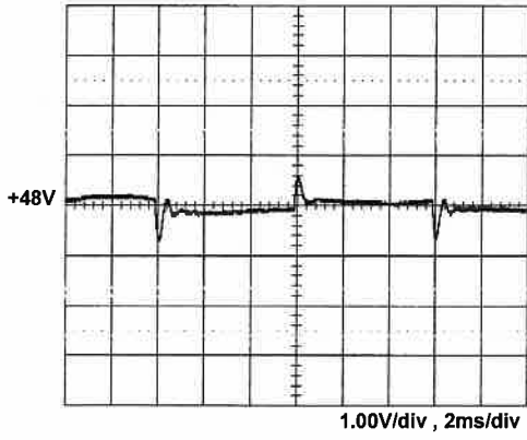
+48V step from 0.75A to 2.5A
