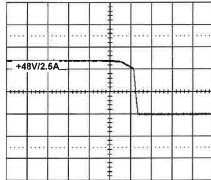
20.0v/div , 20ms/div
