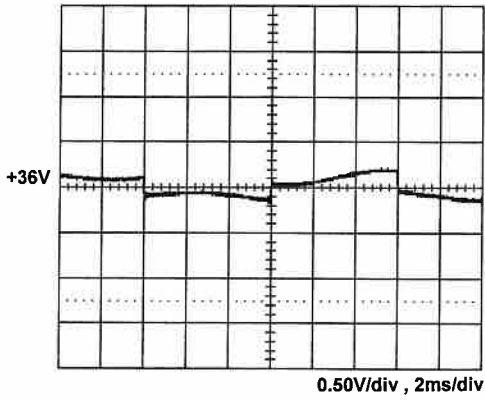
+36V step from 0.68A to 3.4A
