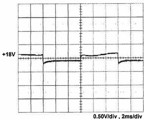
+18V step from 1.32A to 6.6A
