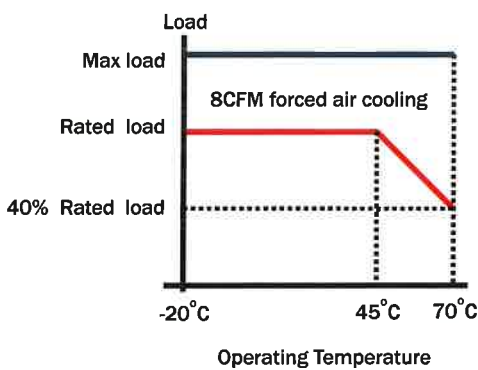
Output derating graph
