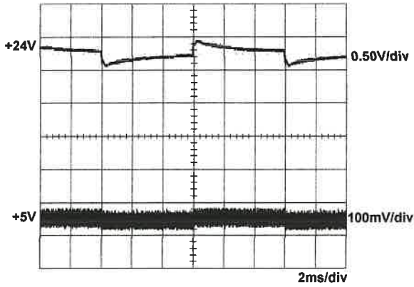
+24V step from 1A to 5A other output at 60% load
