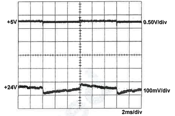
+5V step from 0.9A to 4.5A other output at 60% load
