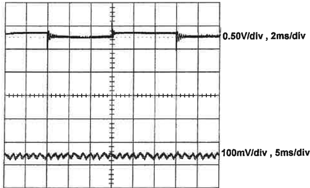
+12V step from 6.67A to 33.33A +5Vsb / 0.6A
