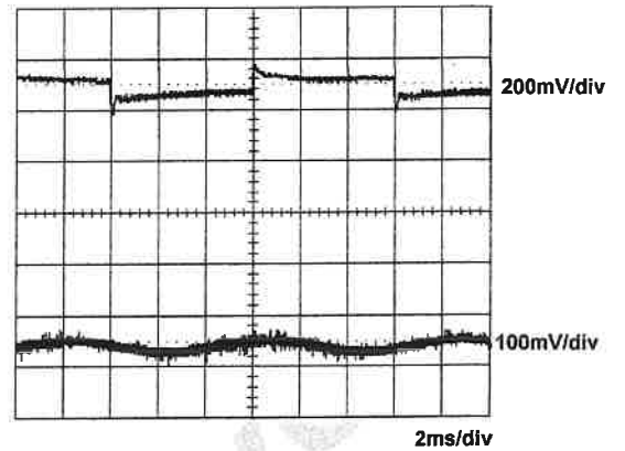
+5Vsb step from 0.2A to 1A +12V/20A
